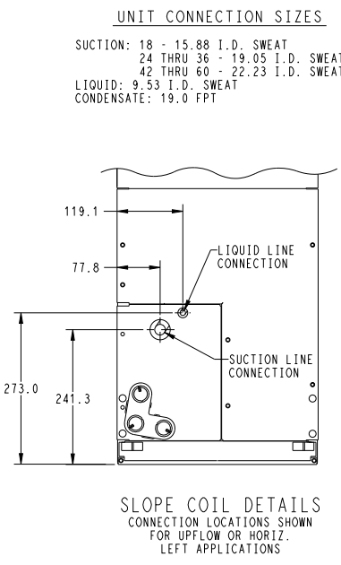
Fig. 3 – FHMA5 - Metric (sheet 1)
