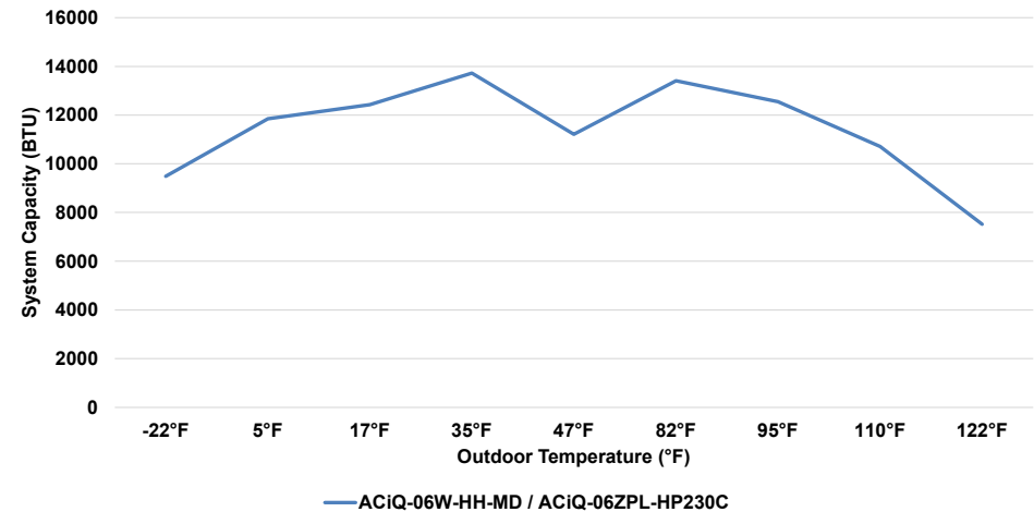
6K Wall Mounted Air Handler & 6K Extreme Heat Single-Zone Condenser Cooling Performance at 80°F Setpoint
