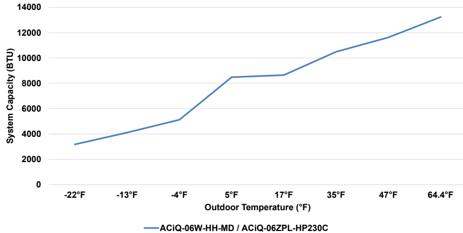
6K Wall Mounted Air Handler & 6K Extreme Heat Single-Zone Condenser Heating Performance at 70°F Setpoint
