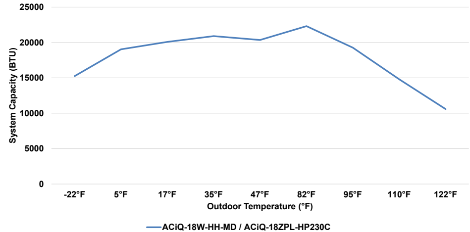
18K Wall Mounted Air Handler & 18K Extreme Heat Single-Zone Condenser Cooling Performance at 80°F Setpoint
