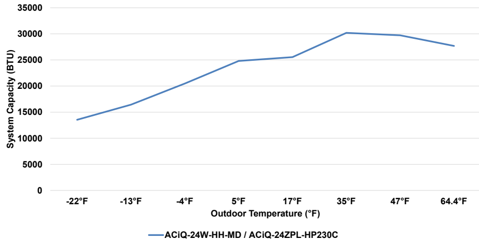
24K Wall Mounted Air Handler & 24K Extreme Heat Single-Zone Condenser Heating Performance at 70°F Setpoint
