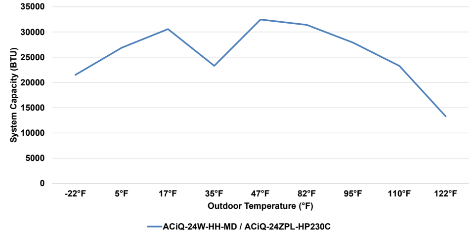
24K Wall Mounted Air Handler & 24K Extreme Heat Single-Zone Condenser Cooling Performance at 80°F Setpoint
