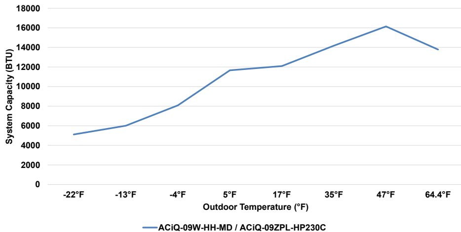
9K Wall Mounted Air Handler & 9K Extreme Heat Single-Zone Condenser Heating Performance at 70°F Setpoint
