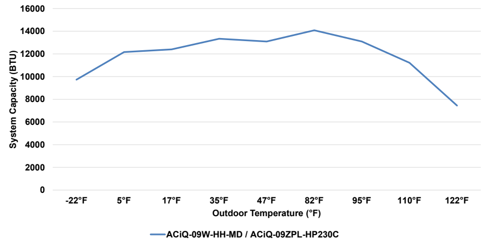
9K Wall Mounted Air Handler & 9K Extreme Heat Single-Zone Condenser Cooling Performance at 80°F Setpoint
