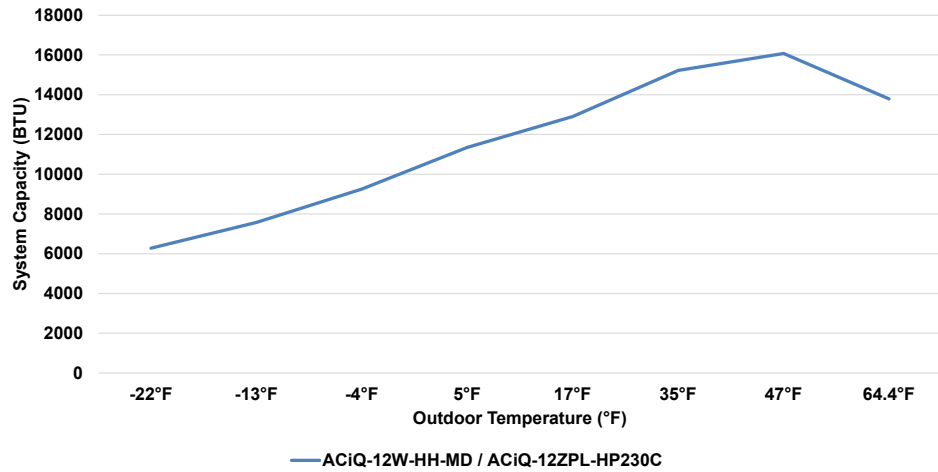
12K Wall Mounted Air Handler & 12K Extreme Heat Single-Zone Condenser Heating Performance at 70°F Setpoint
