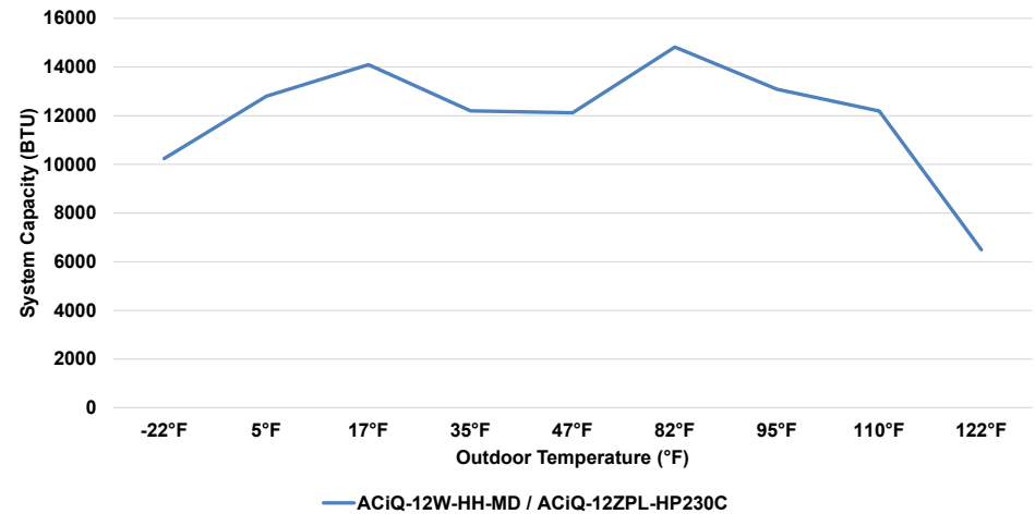
12K Wall Mounted Air Handler & 12K Extreme Heat Single-Zone Condenser Cooling Performance at 80°F Setpoint
