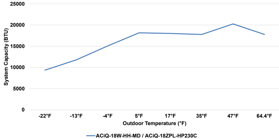
18K Wall Mounted Air Handler & 18K Extreme Heat Single-Zone Condenser Heating Performance at 70°F Setpoint
