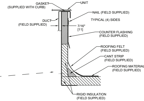
VIEW "B" CORNER DETAIL
