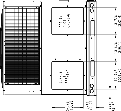
REAR VIEW
