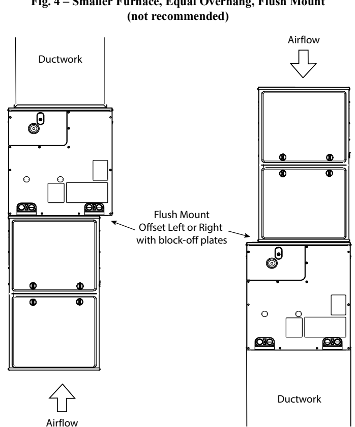
Fig. 5 – Smaller Furnace, Offset, Flush Mount Right or Left (not recommended) A221113A
